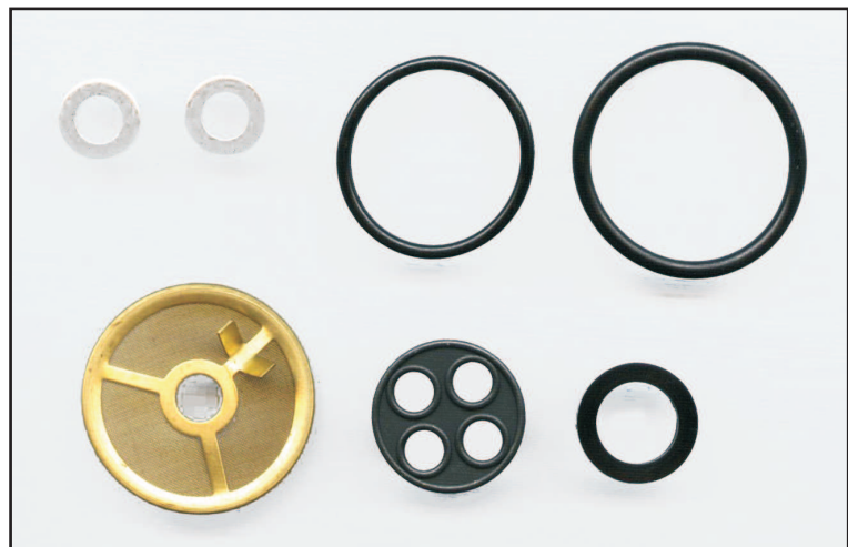
Dichtscheibe Ø = 20,0mm - Sieb Ø = 31,0mm
